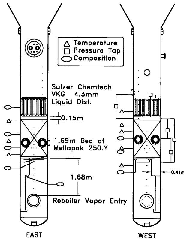
Figure 6. Mellapak 250.Y test 1.69 m bed (chordal block)
