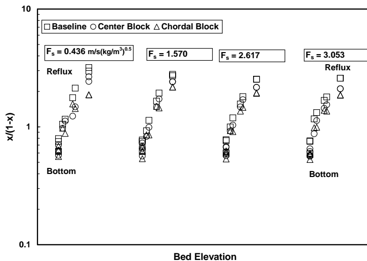
Figure 12 Composition profiles of p-xylene, o/p xylene, 0.13 bar, total reflux
