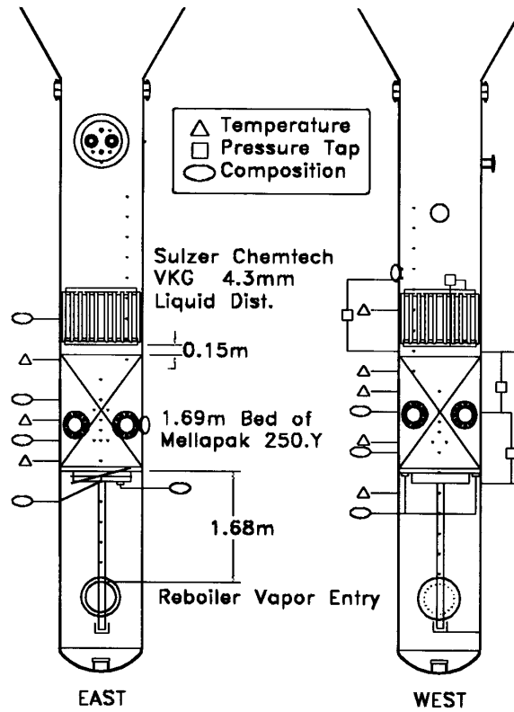
Figure 4. Mellapak 250.Y test 1.69 m bed (center block)
