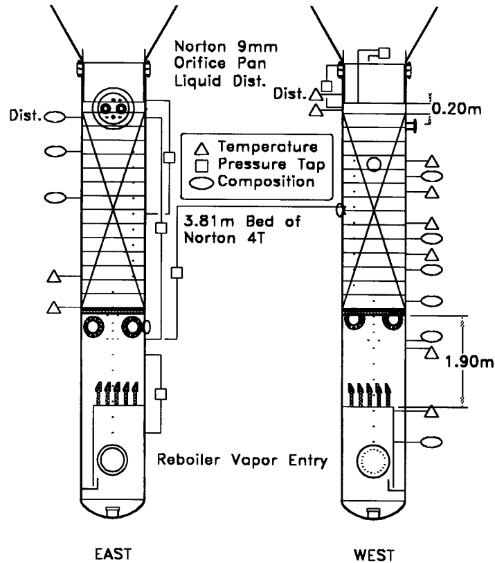
Figure 8. Intalox 4T test 3.81 m bed
