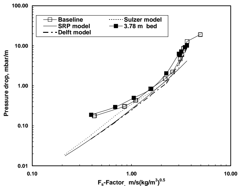
Figure 10. Mellapak 250.Y bed pressure drop, o/p xylene, 0.13 bar, total reflux
