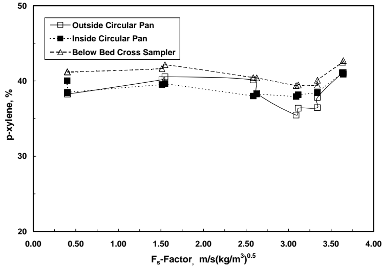
Figure 13 Liquid composition at different locations, o/p xylene, 0.13 bar, total reflux
