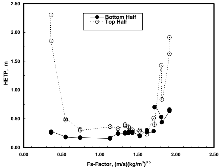
Figure 17 Bed efficiency iC_4/nC_4 system, 11.4 bar, total reflux
