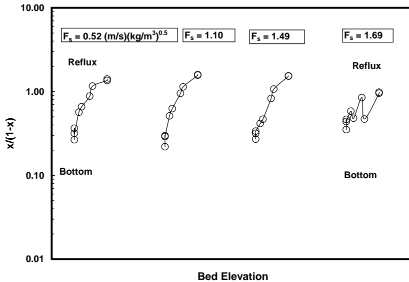
Figure 18 Composition profiles of iC_4 , iC_4/nC_4 system, 11.4 bar, total reflux
